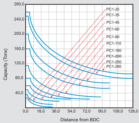
Stroke-Capacity Curve
